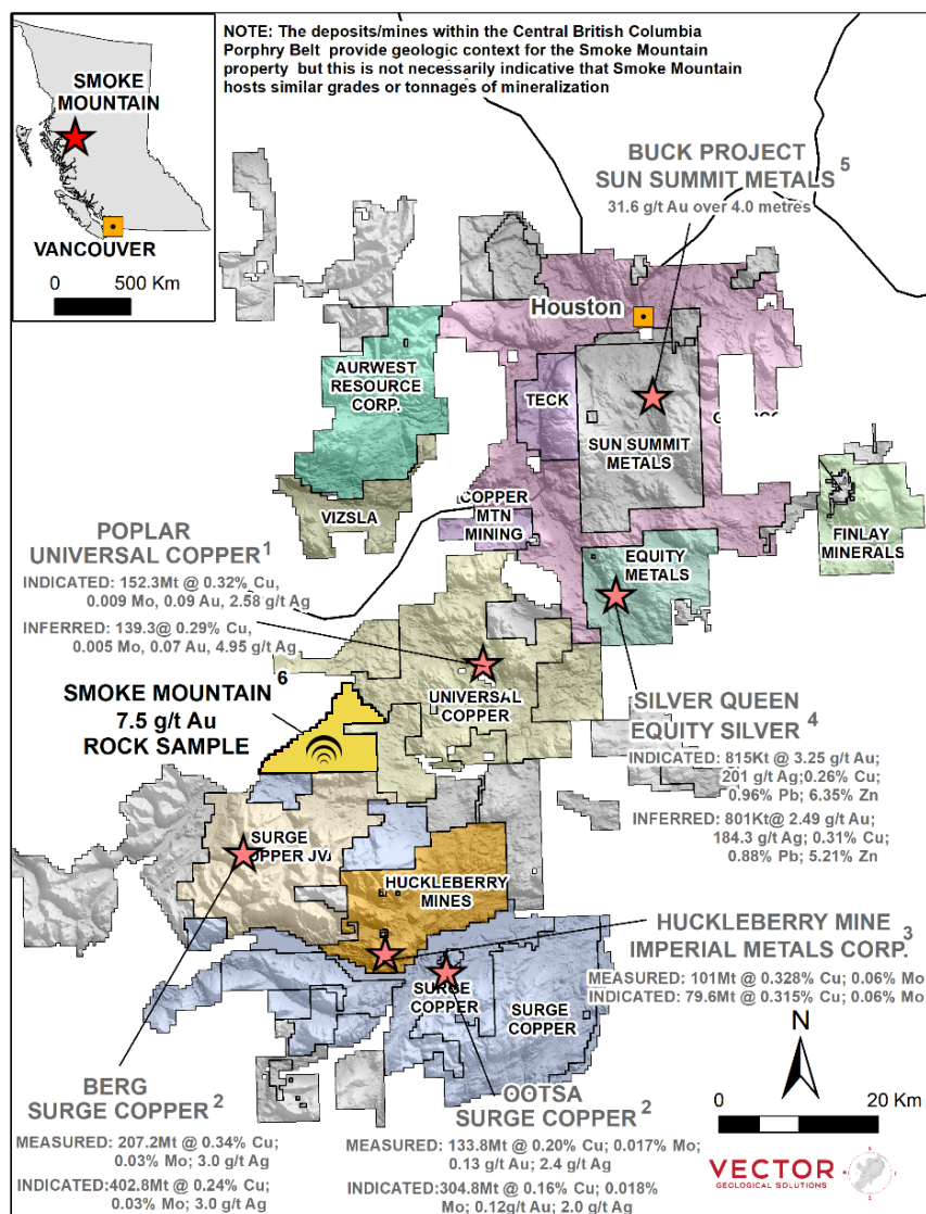
Figure 1. The location of the Smoke Mountain property in the Central BC porphyry-epithermal belt. Note: The deposits, mines, and prospects in this part of BC provide geologic context for the Smoke Mountain property, but these are not necessarily an indication that the Property hosts similar grades or tonnages of mineralization.
