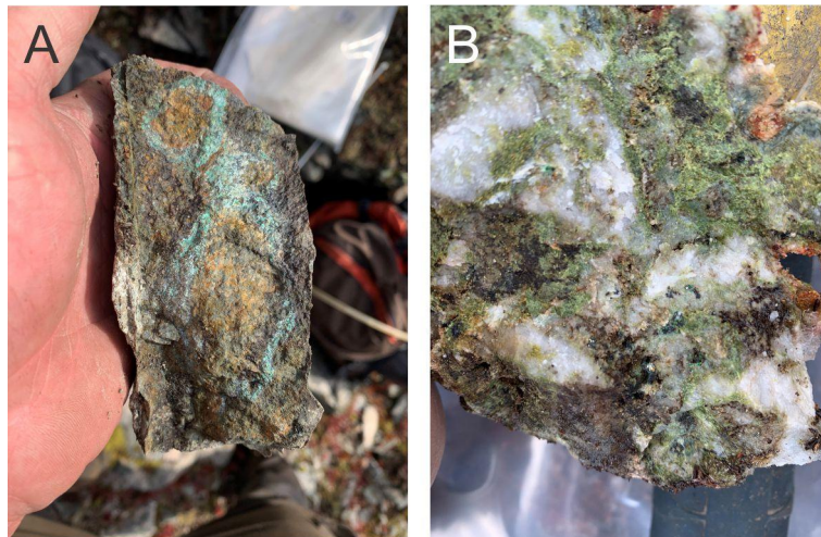
Figure 1. Selected samples from initial mapping, prospecting, and sampling at GoldHaven's Smoke Mountain Project, located the Central British Columbia porphyry/polymetallic Belt
